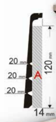
Plinthe de recouvrement : 14x120x2200 mm Covering skirting Rodapié de solapamiento
