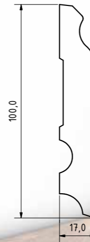
Plinthe structurée : 17x100x2600 mm Skirting with molding Rodapié con moldura
